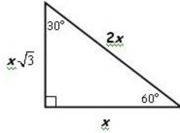
30-60-90 Triangle:
